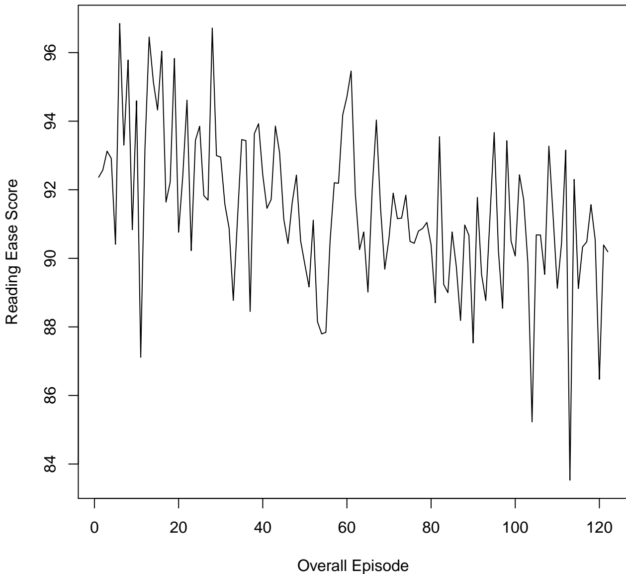
Line Plot of Reading Ease Score by Episode
