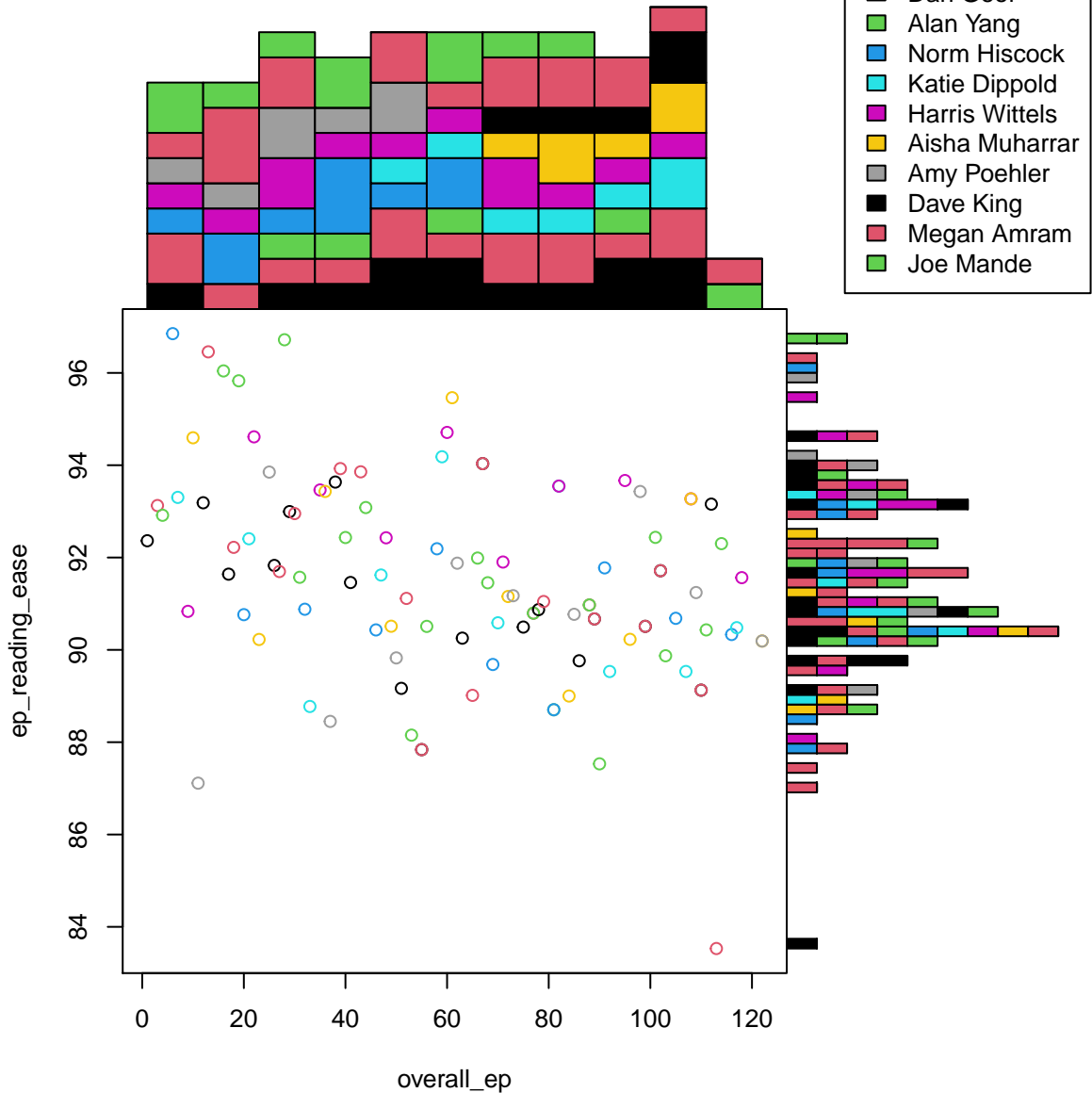
Scatterplot of overall_ep against ep_reading_ease by writers_w_5
