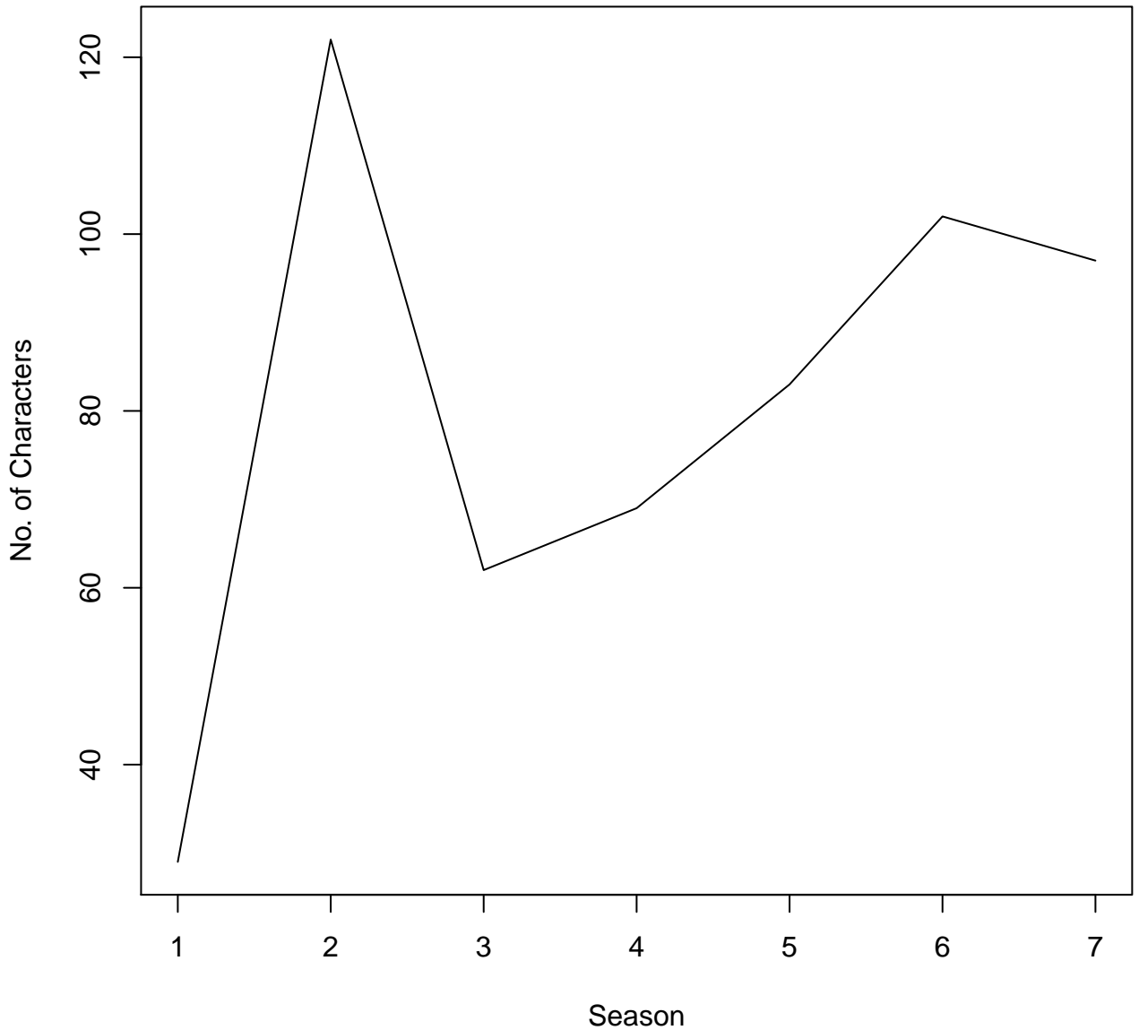
Line Plot of Amount of Characters by Season
