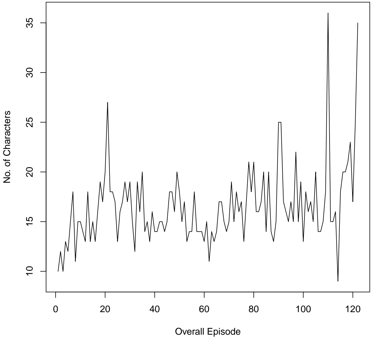
Line Plot of Amount of Characters by Episode
