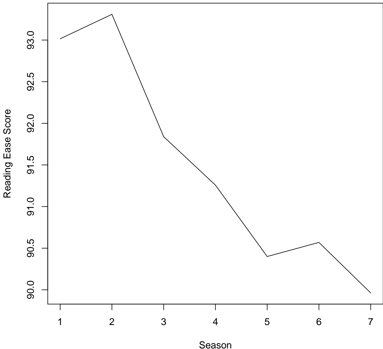
Line Plot of Reading Ease Score by Season
