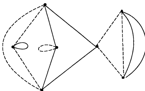
Figure 4. The graph G_2 .
