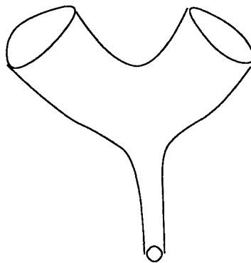
Figure 6. One Y -piece.
