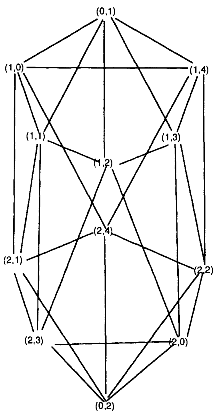
Figure 2. The graph G'_5 .
