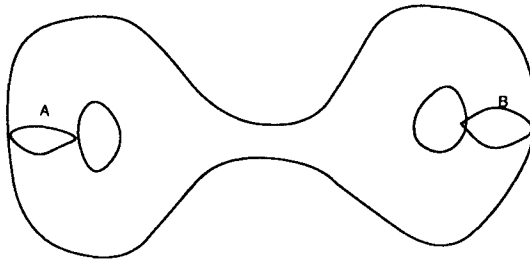
Figure 5. The surface S_0 .
