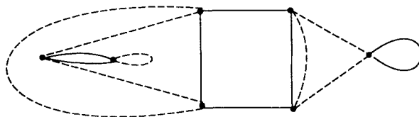
Figure 3. The graph G_1 .
