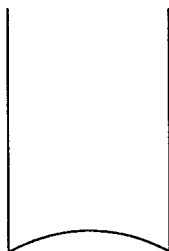
Figure 1. The fundamental domain.
