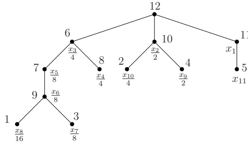
FIGURE 7. Coordinates in a tree.
