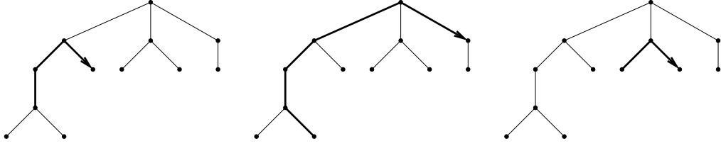
FIGURE 3. Cane paths in a tree.
