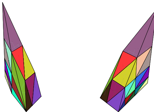
FIGURE 2. A triangulation of the Tutte polytope T_3(q, t) from two angles.
