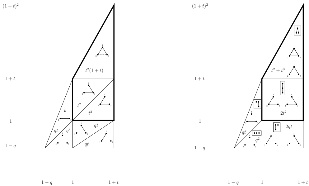
FIGURE 1. A triangulation and a subdivision of the Tutte polytope T_2(q, t) .
