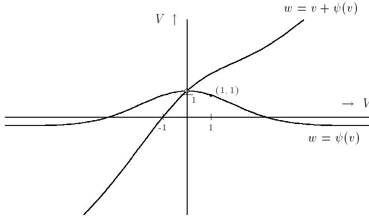
FIG. 1. \psi and \text{id} + \psi on V^* .
