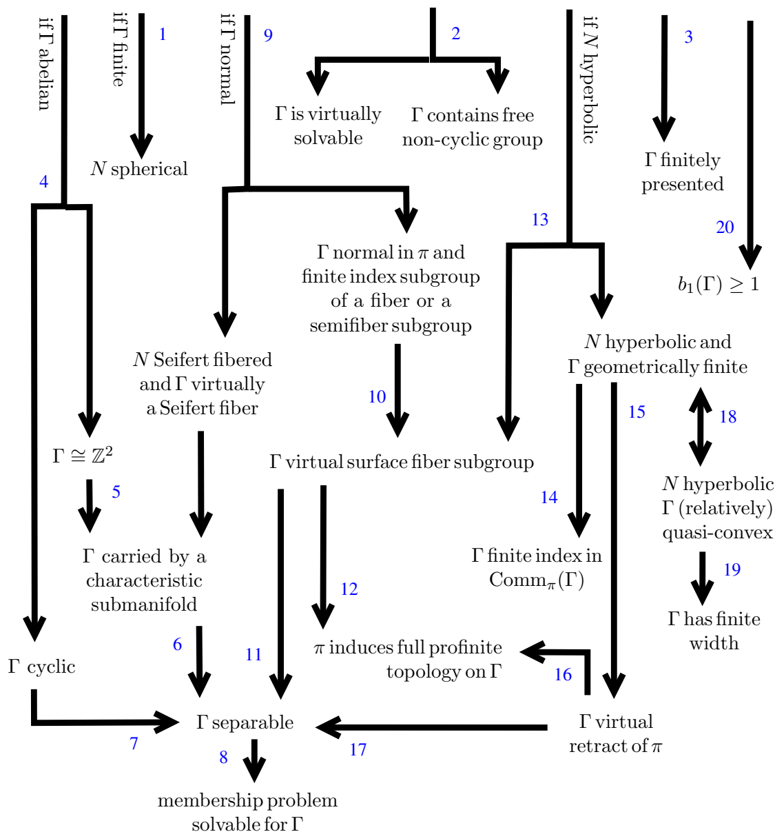
Diagram 5. Subgroups of 3-manifold groups.
