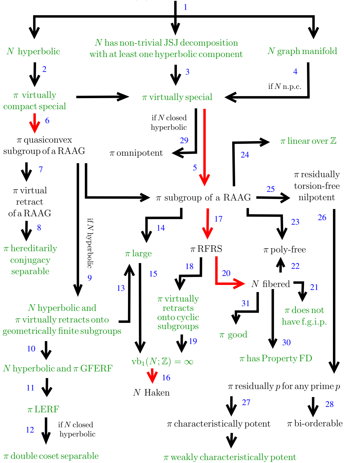
Diagram 4. Consequences of being Virtually (Compact) Special.
