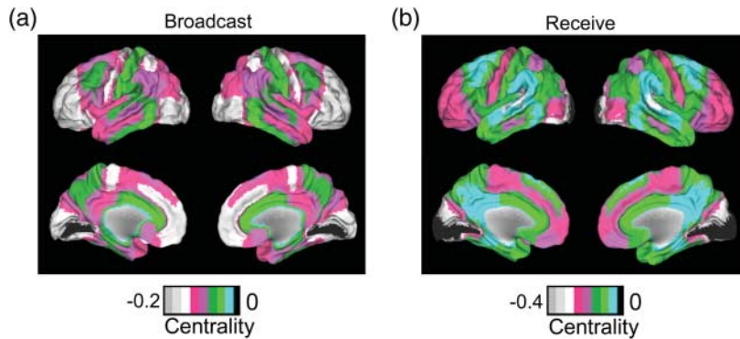
FIG. 2. Anatomical distribution of decrease over time (Day 3 minus Day 1) in broadcast and receive centralities. Broadcast (a) and receive (b) centralities with normalized centrality vectors over subjects.
