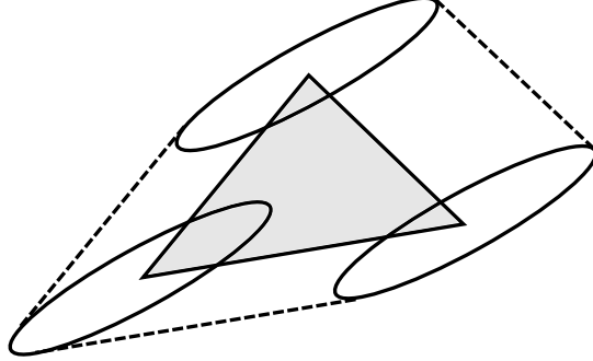
FIG. 1. An illustration of the argument underpinning the proof of Lemma 3.11. Here the shaded triangle corresponds to the convex polygon U while the ellipses stand for the set V . Note that the dashed lines are just translates of the sides of the triangle.
