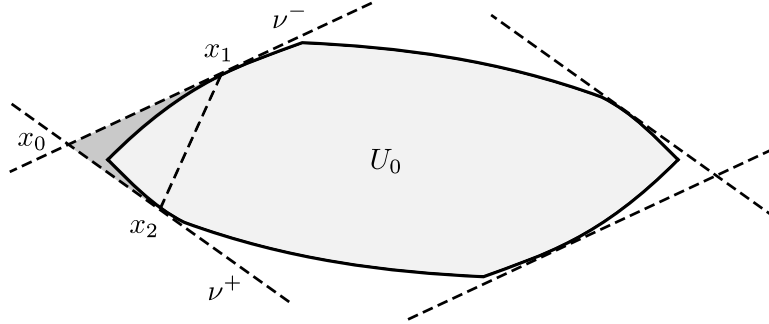
FIG. 2. The construction of U in the second part of the proof of Theorem 1.7. The underlying set is necessarily symmetric with respect to x \mapsto -x , so if a corner can be added on one side of the set, a symmetric corner would appear on the other side as well.
