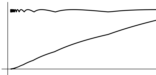
FIG. 2 The graph of the \beta \rightarrow \infty limit of r \mapsto \phi_\beta(r) (top curve) and the corresponding limit for L_\beta(r) := (\log r)^\Delta \phi_\beta(r) (bottom curve) for the choices d = 1 and s = 1.6 . (The adjustment due to u(\beta) is hidden in the parametrization of the horizontal axis.) The bottom graph touches down on the horizontal axis at r = 1 . The mild cusps at the points \{e^{\gamma^n} : n \in \mathbb{Z}\} arise from the function on the right of (1.10) having unequal derivatives at t = 0 and t = 1 .
