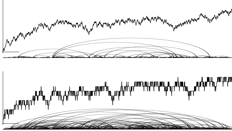
FIG. 1 Top figure: A plot of the chemical distance from the origin to points in \{1, \dots, 2000\} in a sample of long-range percolation on \mathbb{Z} with q(x) := |x|^{-s} (for |x| > 1 ) and parameters s := 1.5 and \beta := 1 . The arcs below depict the edges in the underlying graph. Bottom figure: A corresponding plot for a sample with s := 1.5 but \beta := 5 . Note that the distance drops at the points where a long edge lands. The chemical distance plots are not to scale.
