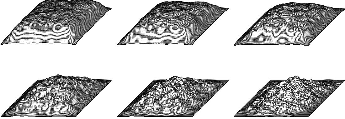
FIG. 2 Empirical plots of x \mapsto \rho^D(x,t) obtained from a set of about 100000 samples of the maximum of the DGFF on a 100 \times 100 square. The plots (labeled left to right starting with the top row) correspond to t increasing by uniform amounts over an interval of length 3 with t in the fourth figure set to the empirical mean. A certain amount of smoothing has been applied to eliminate discrete effects.
