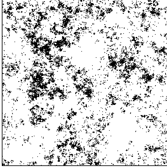
FIG. 3 A sample of the level set for the DGFF on a 500 \times 500 square corresponding to values above 1/3 of the absolute maximum (which occurs at height 8.17 in this sample). The fractal, and highly-correlated, nature of this set is quite apparent. Level sets for higher cutoffs become increasingly sparse and thus difficult to visualize.
