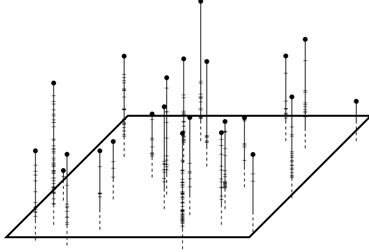
FIG. 1 An illustration of the limit (2.5) of the unstructured point process \eta_N^D for D being a unit square. The “notches” on the vertical lines mark the locations of sample points of an individual cluster. Only the points above a certain (arbitrary) base value are included. The top values in the clusters (marked by bullets) are distributed according to the Cox process in (1.6).
