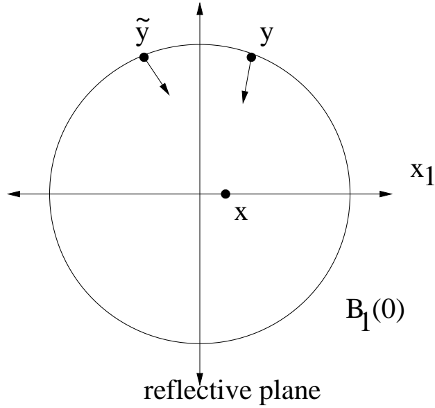
Figure 1: Figure for Lemma 8
