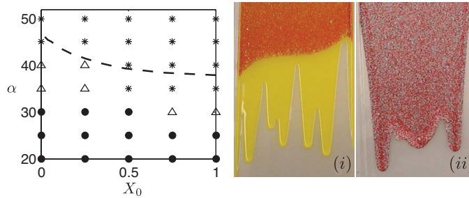
Fig. 5 (Left) Bifurcation \alpha_A(X_0) (dashed line) between settled and ridged regimes for fixed \phi_0 = 0.4 with varying \alpha and X_0 . The symbols indicate experimental results identified as ridged (star) or settled (circle). The triangles mark results for which the particles did not equilibrate in the duration of the experiment. (Right) Photographs of the experiment in the settled and ridged regimes are shown on the right for experimental parameters, (i) \alpha = 20^\circ , X_0 = 0.5 and (ii) \alpha = 50^\circ , X_0 = 0.5 .
