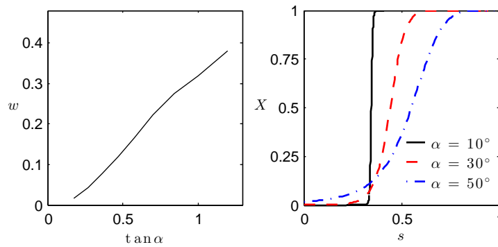
Fig. 3 Dependence of the width w of the mixing region (where 0.05 < X < 0.95 ) on \tan \alpha ; the relationship, shown on the left, is approximately linear. The right panel shows the X profiles for \alpha = 10, 30, 50 deg.
