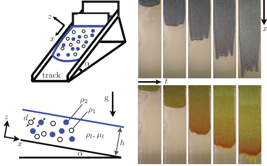
Fig. 1 (top left) Schematic of the experimental apparatus; (bottom left) The thin film of fluid of \rho_l and \mu_l that contains two particle species of equal diameter d and variant densities, such that \rho_2 > \rho_1 > \rho_l . Two sets of experimental results are shown on the right. In the bottom right panel, as time evolves (images from left to right), clear fingers form on the flow front, indicating that both particle species have settled to the channel walls with a clear fluid layer on top that moves ahead. On the other hand, the particles appear to remain aggregated and well-mixed on the front in the ‘ridged’ regime, as shown in the top right panel.
