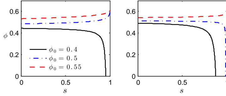
Fig. 2 Transition from settled to ridged solutions in \phi for the monodisperse system, for X = 1 (left) and X = 0 (right). The critical concentrations are \phi_{c,1} = 0.459 and \phi_{c,2} = 0.521 .
