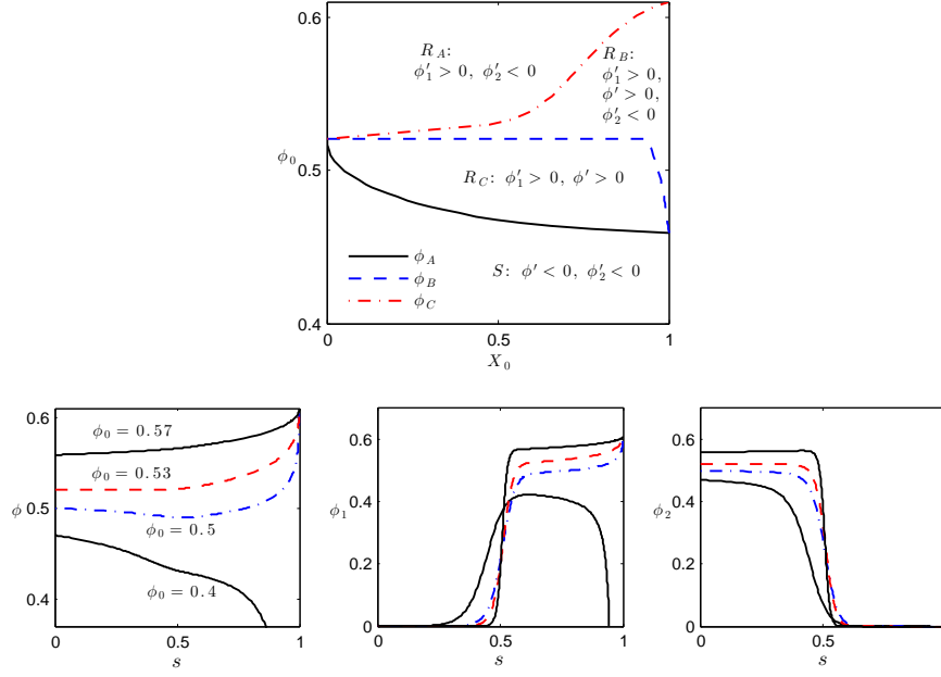
Fig. 4 The left panel shows a phase diagram of solution regimes determined by total and relative concentrations (X_0, \phi_0) , separated by transition curves \phi_A, \phi_B and \phi_C . Profiles in each region are shown below, for total concentration \phi (left) and for the individual concentrations \phi_1, \phi_2 .
