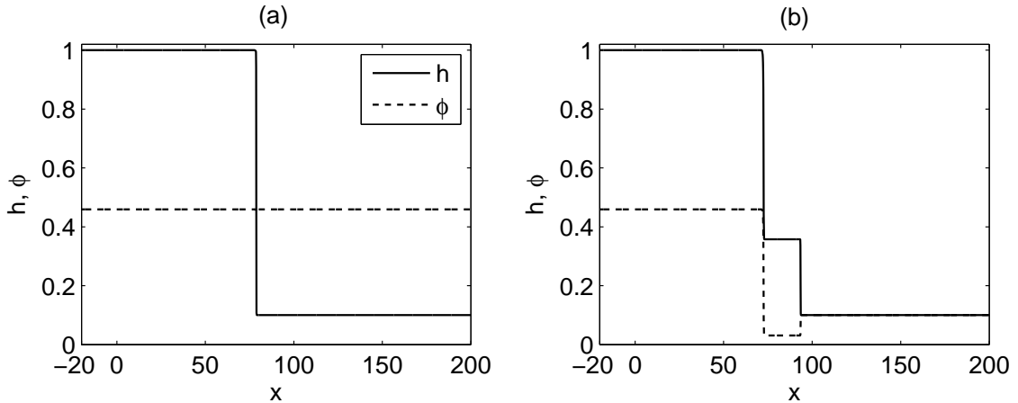
Fig. 12 Numerical solution of the film thickness (solid line) and the particle volume fraction (dashed line) at t = 2000 . In both panels, the left and right states are chosen as h_- = 1 and h_+ = 0.1 , respectively and the left state for \phi is 0.4593, which is equivalent to the critical concentration, \phi_c according to Eq. (17). In panel (a) the initial condition for \phi is given by Eq. (37) and in (b), we use Eq. (38) with \phi_+ = 0.1 . Here, the domain length is \mathcal{L} = 220 and the mesh size used is dx = 0.1 .
