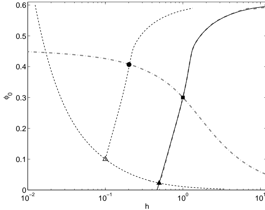
Fig. 6 Shock and rarefaction curves for the system. Here, the Rankine-Hugoniot locus calculated using Eq. (26) shows 1-shock connections (solid lines) from the fixed state (1, 0.3) (■) and shock connections (dashed lines) from a second fixed state (0.1, 0.1) (△). 1- and 2-rarefaction integral curves at (1, 0.3) are shown by thick, dot-dashed, gray lines. We mark two intersection points: one given by the shock-shock connections (shown with a ▲) and another given by the shock-rarefaction connections (shown with a ●). We note that the 1-shock and 1-rarefaction curves for the state (1, 0.3) overlap. Numerical simulations show that, starting with (1, 0.3) as the upstream state give a shock-shock solution (see Fig. 8 for a representation of the numerical solution) while, starting with (1, 0.3) as the downstream state the solution is described by a 1-shock, 2-rarefaction wave (see Fig. 14). The intersection points given by the markers ▲ and ● match the flat states shown in the numerical simulations in Figs 8 and 14, respectively.
