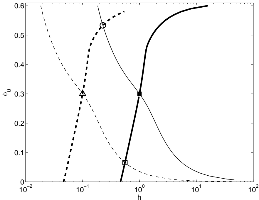
Fig. 4 The Rankine-Hugoniot locus calculated using Eq. (26) showing 1-shock (thick, solid lines) and 2-shock (thin, solid lines) connections from an upstream state (h_-, (\phi_0)_-) = (1, 0.3) (■) and 1-shock (thick, dashed lines) and 2-shock (thin, dashed lines) connections from a precursor state (h_+, (\phi_0)_+) = (0.1, 0.3) (△). The intersections points show the possible intermediate states which are calculated as (h_i, (\phi_0)_i) = (0.56, 0.065) (□) and (h_i, (\phi_0)_i) = (0.23, 0.53) (○).
