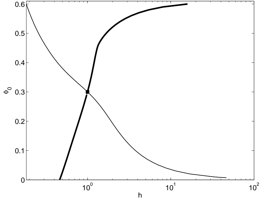
Fig. 3 Phase diagram showing the Rankine-Hugoniot locus calculated using Eq. (26). The locus shows all possible 1-shock (thick line) and 2-shock (thin line) connections from the fixed state chosen as h_- = 1 and (\phi_0)_- = 0.3 (the fixed states are indicated by the square marker).
