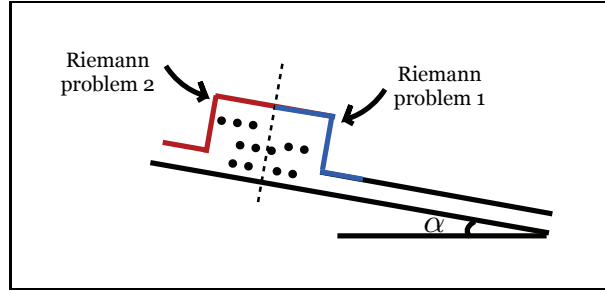
Fig. 7 Initialization of numerical simulations. We tackle two Riemann problems to identify all shock and rarefaction connections for the 2 \times 2 system of conservation laws. In ‘Riemann Problem 1’ h_- > h_+ while in ‘Riemann Problem 2’, h_- < h_+ . The initial conditions for the particle volume concentration vary from a uniform concentration along all x to a step-up or step-down function similar to the two Riemann problems shown in this figure.
