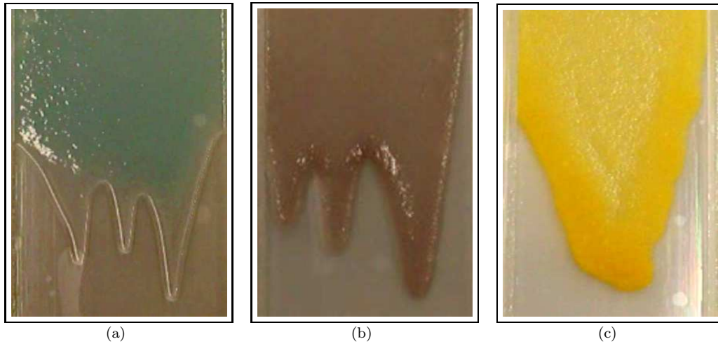
Fig. 1 Flow regime patterns emerging from a fixed volume of silicon oil laden with small ( \sim 300 \mu m ), negatively buoyant glass beads. The experimental apparatus consists of a rectangular plane, which is 90 cm long by 14 cm wide and, in the pictures shown here, it is inclined at an angle of 30^\circ . In (a)-(c), the particle volume fraction is set as 0.25, 0.35 and 0.5 corresponding to the ‘settled’, ‘well-mixed’ and ‘ridged’ regime, respectively. In the ‘settled’ regime, clear fluid flows over the particle-rich fluid while in the ‘ridged’ regime, the particles accumulate at the front indicated by the darker yellow color in panel (c). The middle panel shows an intermediate regime where the particles remain well mixed in the fluid. The images show the patterns at their fully developed state captured at 2, 4 and 20 minutes after the onset of the experiment in panels (a)-(c), respectively. The experiments were run in the Applied Mathematics Laboratory at University California, Los Angeles (UCLA) (see [9, 10] for more details on the experiments).
