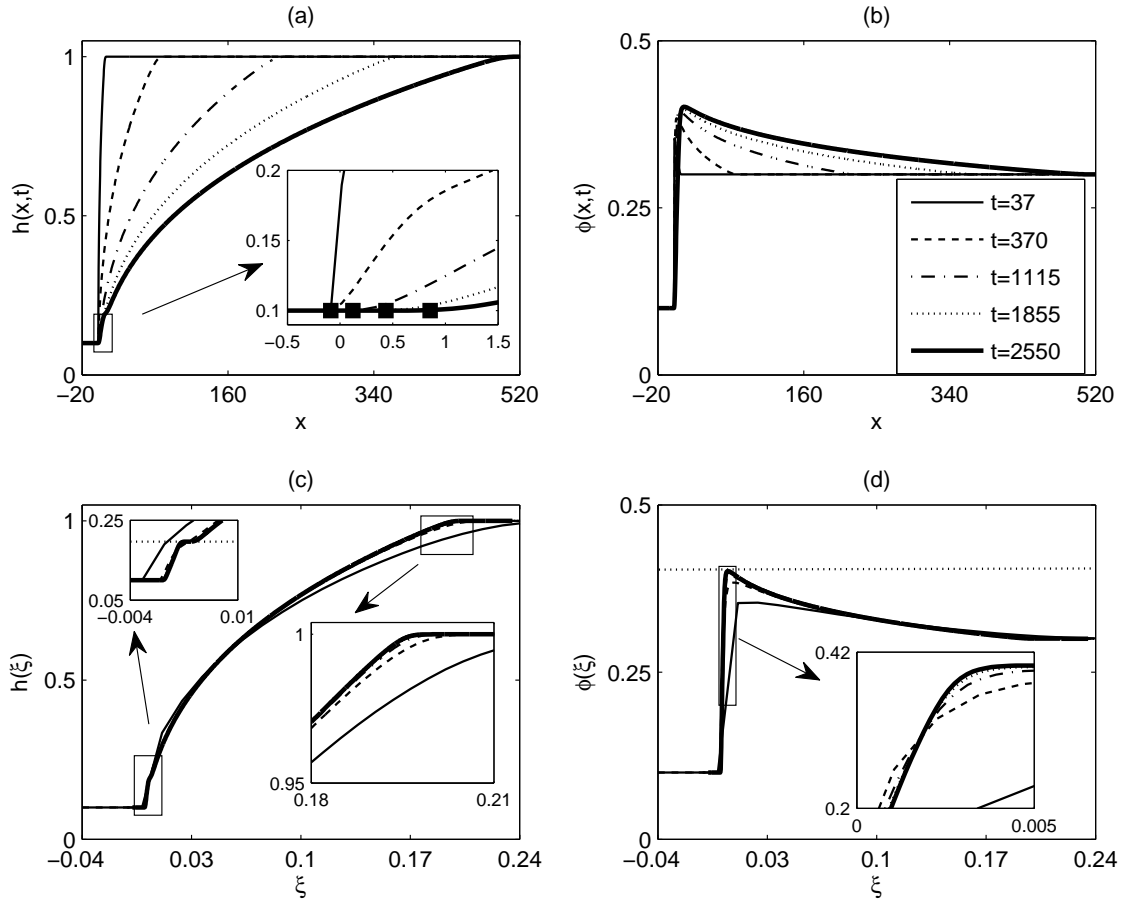
Fig. 14 Numerical simulations showing the evolution of h [panel (a)] and \phi [panel (b)] starting from Eqs. (36) and (37) for h and \phi , respectively. The left states are chosen as (0.1, 0.1) and the right states as (1, 0.3) ; the averaged particle volume fraction is fixed at 0.1 at the left boundary. The final solution time is shown with a thick, solid line at t = 2550 while the legend in panel (b) shows the times for all the solutions. From left to right, the square markers shown in the insert in panel (a) illustrate that the x -position of the upstream shock is advancing in x with time, albeit rather slowly. Panels (c) and (d) depict plots of the film thickness and the particle volume fraction, respectively, against the rescaled variable \xi = x/t showing the formation of a 1-shock and a 2-rarefaction wave; the latter is indicated by the complete overlap of the late-time solutions. The different line types correspond to the legend shown in panel (b). The leftmost insert in panel (c) depicts the formation of the intermediate state connecting the shock and rarefaction wave where the horizontal, dotted line shows that the intermediate value for h is at h = 0.2 . The intermediate state for \phi is shown in panel (d) with a horizontal, dotted line at \phi = 0.4 .
