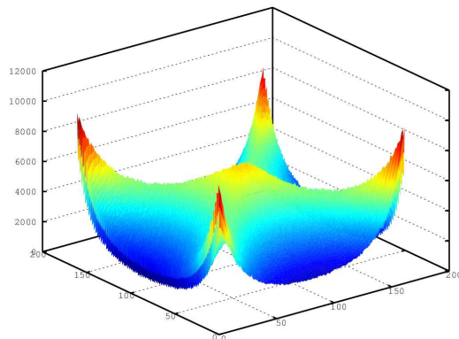
FIGURE 8. Averages of alternating Baxter permutations ( n = 200 ).
