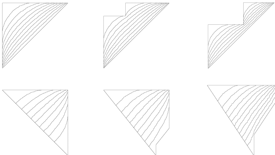
FIGURE 3. Simulations for k = 300 . Left column: \text{SYT}(\delta_k) and \text{ShSYT}(\varrho_k) . Middle column: \text{SYT}(\delta_k/b^a) and \text{ShSYT}(\varrho - \tau^{a,b}) with (a, b) = (60, 100) . Right column: \text{SYT}(\delta_k/b^a) and \text{ShSYT}(\varrho - \tau^{a,b}) with (a, b) = (100, 160) .
