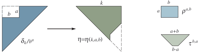
FIGURE 1. Main bijection \varphi : \text{SYT}(\delta_k/b^a) \longrightarrow \text{ShSYT}'(\eta) .
