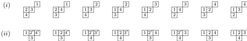
FIGURE 2. The sets (i) \text{SYT}(\delta_4/(2)) and (ii) \text{ShSYT}'(\varrho_4 - (2)) , with columns corresponding to our bijection.
