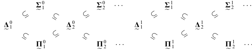
DIAGRAM 1. The finite-order Borel and the projective pointclasses.
