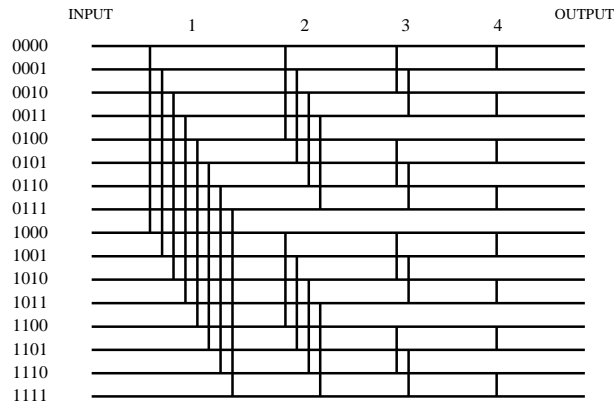
Figure 1. The network \text{CCC}_{16} .
