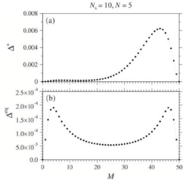
FIG. 7. The overall error of mass-action kinetics. (a) The averaged error in the metastable regime \Delta^* . (b) The averaged error \Delta^{\text{eq}} in the equilibrium limit t \gg \varepsilon^{-1} .
