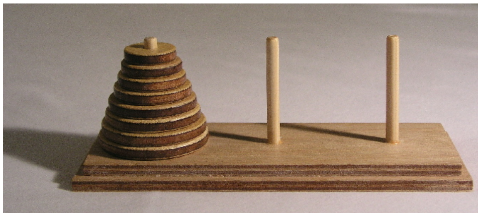
The Hanoi tower with eight disks.
