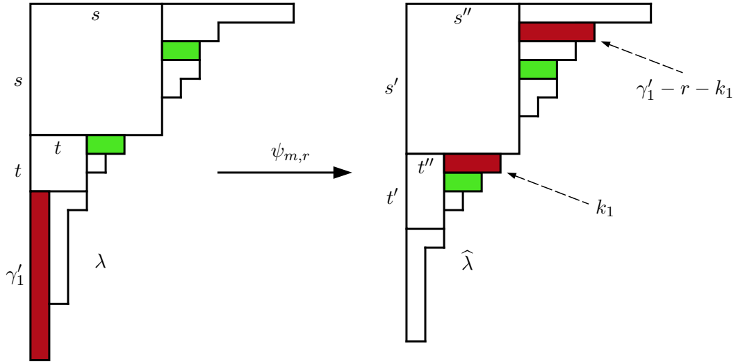
FIGURE 5. An example of the second symmetry bijection \psi_{m,r} : \lambda \mapsto \widehat{\lambda} , where \lambda \in \mathcal{H}_{n,m,\leq -r} , \widehat{\lambda} \in \mathcal{H}_{n',m+2,\geq -r} , for m = 0 , r = 2 , n = 92 , and n' = n - r - 2m - 2 = 88 . Here r_{2,0}(\lambda) = 2 + 2 - 9 = -5 \leq -2 and r_{2,2}(\widehat{\lambda}) = 3 + 4 - 6 = 1 \geq -2 , where \lambda = (14, 10, 9, 9, 8, 7, 7, 5, 4, 3, 3, 2, 2, 2, 2, 1, 1, 1) and \widehat{\lambda} = (13, 10, 9, 8, 8, 7, 6, 6, 5, 4, 3, 2, 2, 1, 1, 1, 1, 1) . Also, s = 7 , s' = s + 1 = 8 , s'' = s' - m - 2 = 6 , t = 3 , t' = 4 , t'' = 2 , \gamma'_1 = 9 , k_1 = 3 , and \gamma'_1 - r - k_1 = 4 .
