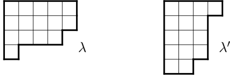
FIGURE 1. Partition \lambda = (5, 5, 4, 1) and conjugate partition \lambda' = (4, 3, 3, 3, 2) .
