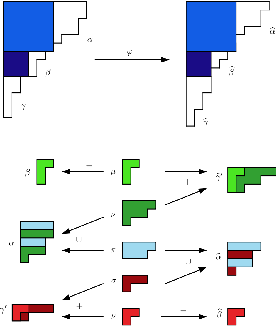
FIGURE 4. An example of the first symmetry involution \varphi : \lambda \mapsto \hat{\lambda} , where \lambda \in \mathcal{H}_{n,0,r} and \hat{\lambda} \in \mathcal{H}_{n,0,-r} for n = 71 , and r = 1 . The maps are defined by the following rules: \beta = \mu , \alpha = \nu \cup \pi , \gamma' = \sigma + \rho , while \hat{\beta} = \rho , \hat{\alpha} = \pi \cup \sigma , \hat{\gamma}' = \mu + \nu . Also, \lambda = (10, 10, 9, 9, 7, 6, 5, 4, 4, 2, 2, 1, 1, 1) and \hat{\lambda} = (10, 9, 9, 7, 6, 6, 5, 4, 3, 3, 3, 2, 2, 1, 1) .
