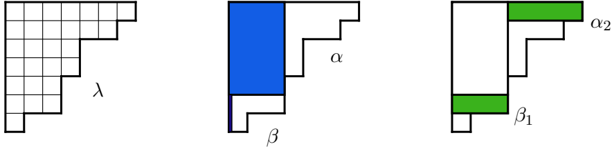
FIGURE 3. Partition \lambda = (7, 6, 4, 4, 3, 3, 1) , the first 2-Durfee rectangle of height s_2(\lambda) = 5 and width 3, and the second 2-Durfee square of height t_2(\lambda) = 2 and width 0. Here the remaining partitions are \alpha = (4, 3, 1, 1) , \beta = (3, 1) , and \gamma which is empty. In this case, we have (2, 2) -rank r_{2,2}(\lambda) = \beta_1 + \alpha_1 - \gamma'_1 = 3 + 4 - 0 = 7 .
