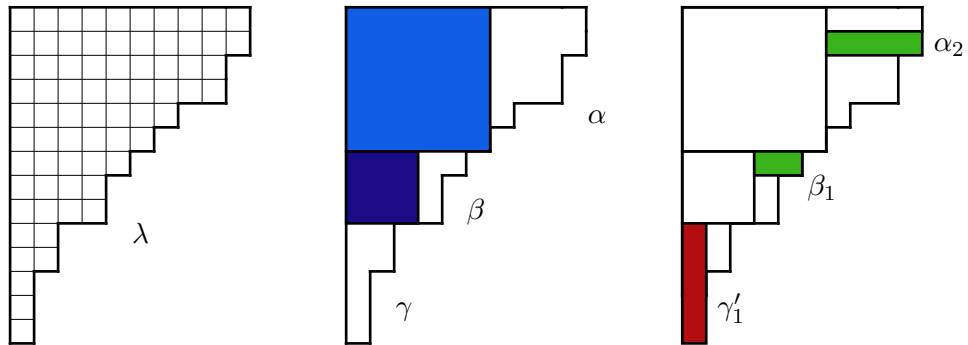
FIGURE 2. Partition \lambda = (10, 10, 9, 9, 7, 6, 5, 4, 4, 2, 2, 1, 1, 1) , the first Durfee square of height s_0(\lambda) = 6 , and the second Durfee square of height t_0(\lambda) = 3 . Here the remaining partitions are \alpha = (4, 4, 3, 3, 1) , \beta = (2, 1, 1) , and \gamma = (2, 2, 1, 1, 1) . In this case, the (2, 0) -rank is r_{2,0}(\lambda) = \beta_1 + \alpha_2 - \gamma_1' = 2 + 4 - 5 = 1 .
