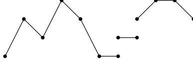
FIGURE 4. A p-sequence with weight q^6 .
