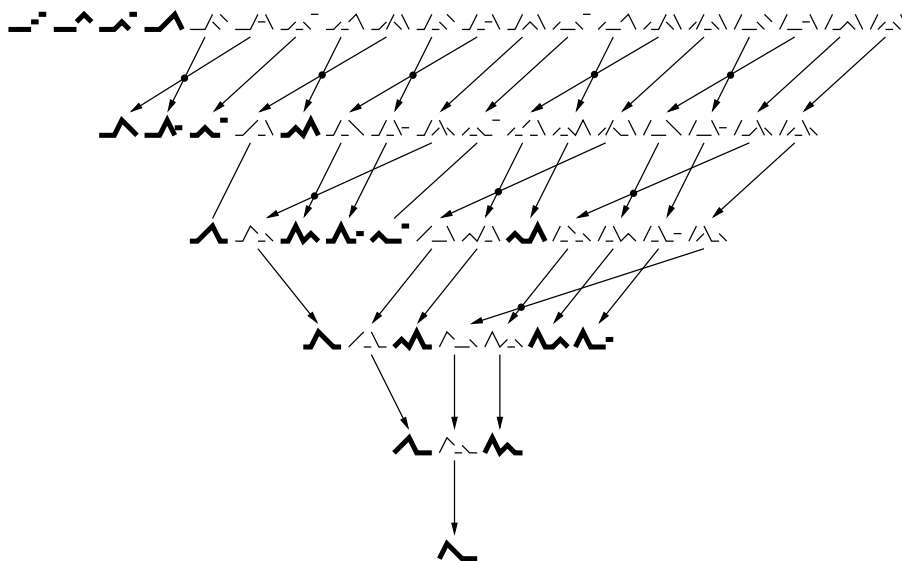
FIGURE 3. Transforming o-sequences into p-sequences via a series of simultaneous switches.
