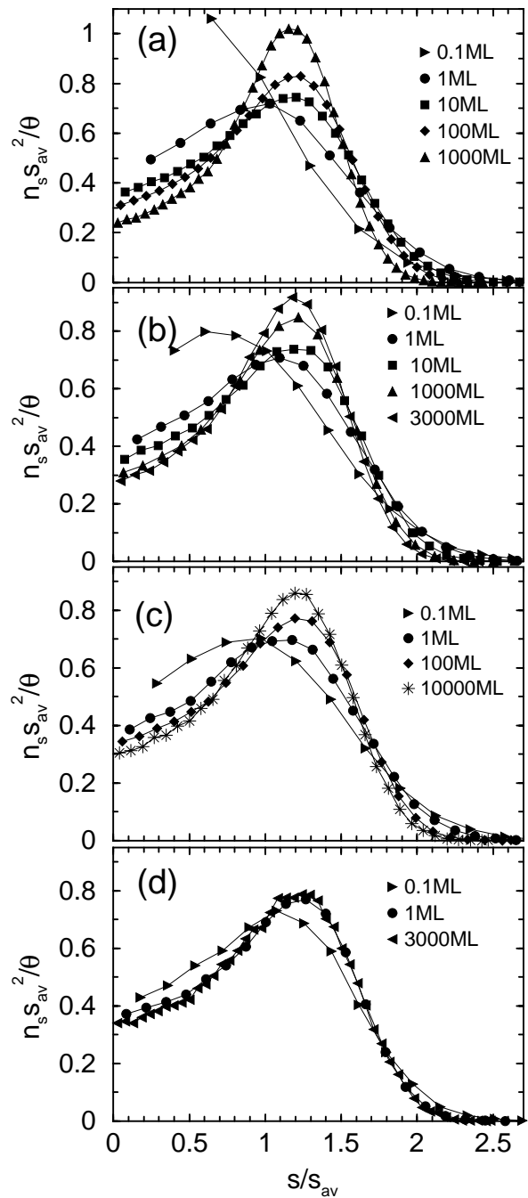
FIG. 1: The scaled ISD for D/F = 10^4 (a), D/F = 10^5 (b), D/F = 10^6 (c), and D/F = 10^7 (d) at different coverages \Theta . Note the different scale in (a).
