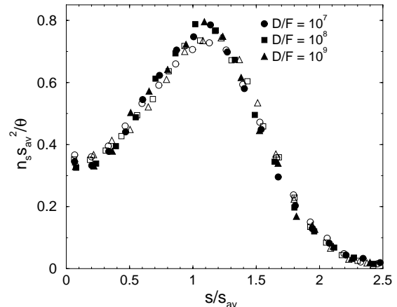
FIG. 4: The scaled ISD in an extended island model at different values of D/F and different coverages. Closed (open) symbols correspond to \Theta = 0.2ML ( \Theta = 0.1ML ).
