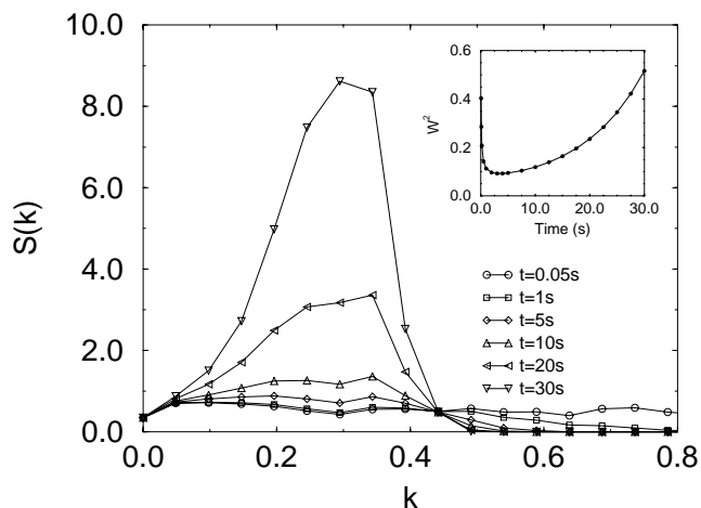
FIG. 2. Evolution of the structure factor S(k) (in arbitrary units) and surface roughness W^2 for the continuum model described by Eq. (2). All simulations were performed on a 128 \times 128 lattice with parameters \alpha = 1.0 , \beta = 50.0 , and \kappa = 5.0 .
