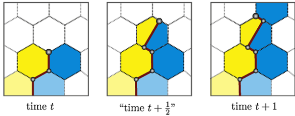
Fig. 5 “Multistep” procedure by which the Exploration Process gets through a mixed hexagon
