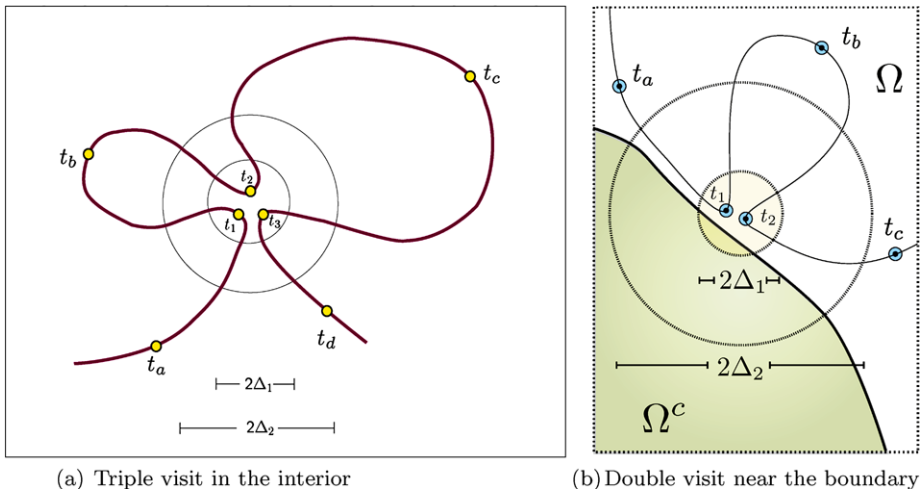
Fig. 1 Atypical behavior of \mu_\varepsilon curves
