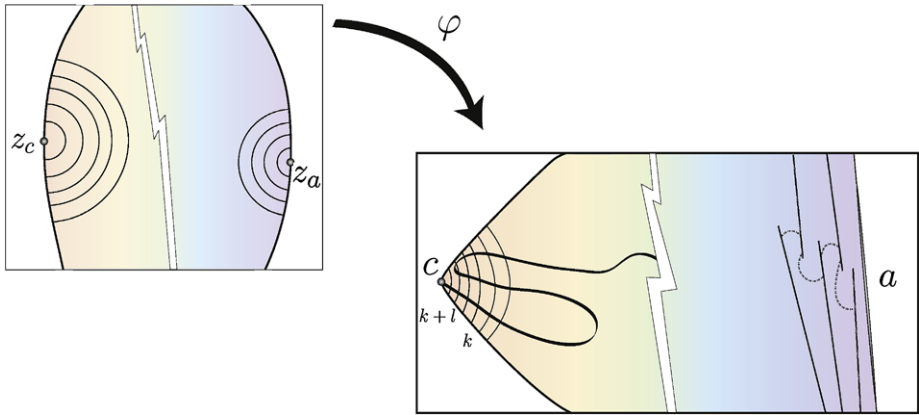
Fig. 2 A jump of magnitude l occurring in the vicinity of the prime end c
