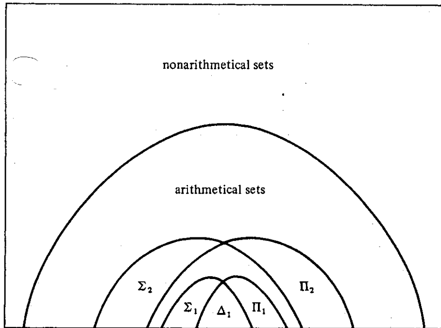
Figure 10. Picture of \mathcal{PN} .
