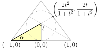
Figure 3: The \beta = 90^\circ case.
