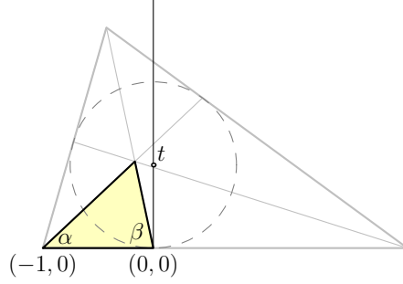
Figure 2: A triangle in standard position.
