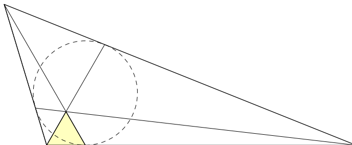
Figure 5: The unique triangle which has an equilateral triangle as a Gergonne daughter.
