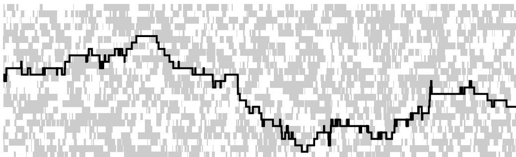
FIG. 1 A path of the random walk X in the dynamical environment composed of independent ON/OFF processes (i.e., the conductances taking values 1 and 0, respectively) with Poisson arrivals of constant (and equal) intensity. The time axis runs horizontally; the shaded areas mark the space-time positions where the corresponding edge is ON. The walk can effectively make a step only across the edges that are ON at that moment of time.
