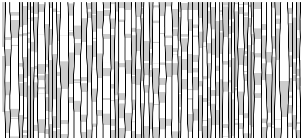
FIG. 2 A sample of the parabolic coordinates for the dynamical environment in Fig. 1. The dark lines mark the “trajectories” t \mapsto \psi(t, x) of individual vertices. The time axis runs upwards this time.
