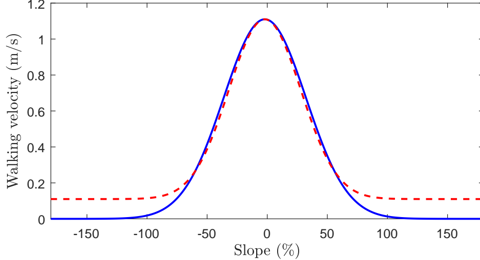
Figure 4: Our velocity function eq. (6) (solid blue line), and the Irmischer and Clarke function (5) (dashed red line). Our velocity function decays to zero for high slopes while the function suggest by Irmischer and Clarke [8] does not.
