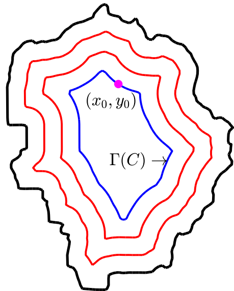
Figure 3: Evolve level sets in from the boundary until the C > 0 such that (x_0, y_0) \in \Gamma(C) .
