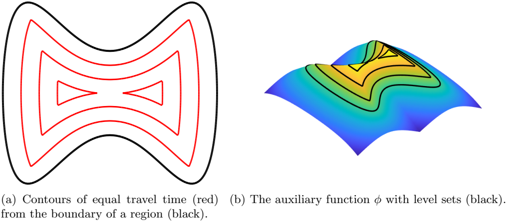
Figure 2: Using the level set method to find contours of equal travel time.
