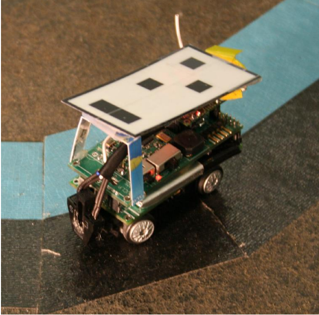
Fig. 2. Autonomous vehicle with downward looking IR device, on colored tape indicating boundary.
