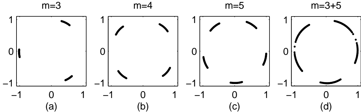
FIGURE 4. Steady-states arising from custom-designer kernels using 200 particles. (a) Pure mode m = 3 instability with g = g^3 + 1.1158g^0 . (b) Pure mode m = 4 instability with g = g^4 + 1.3g^0 . (c) Pure mode m = 5 with g = g^5 + 1.3g^0 . (d) Mixed mode m = 3, 5 instability with g = 1.1225g^3 + g^5 + 1.3g^0 .
