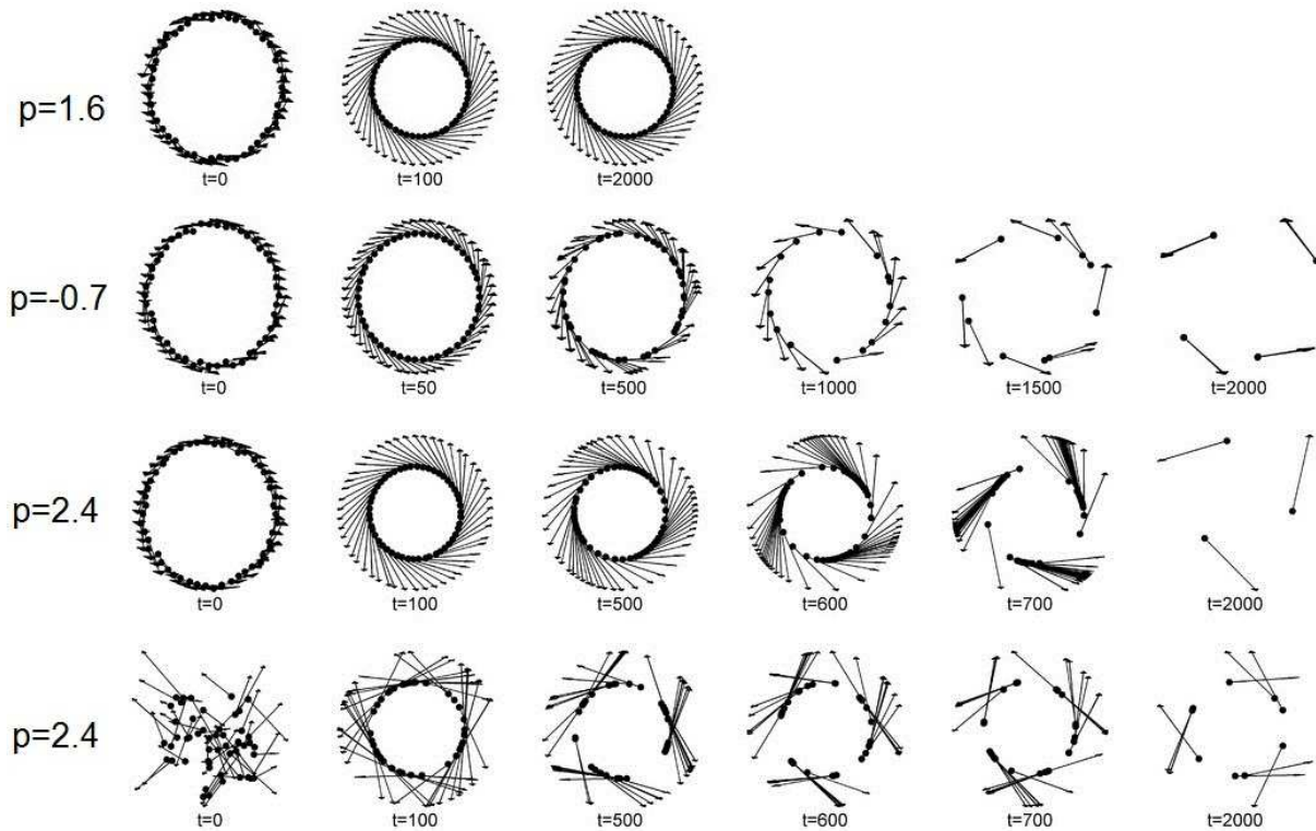
FIGURE 5. Dynamics of the 2nd order model (61) with N = 50 , g(s) = 1 - s^2 and f(r) = -r^p , with p as indicated. Row 1-3: The initial conditions are taken to be a slight random perturbation of a ring of radius one rotating counterclockwise. Row 4: Initial positions and velocities are taken to be random inside a unit square.
