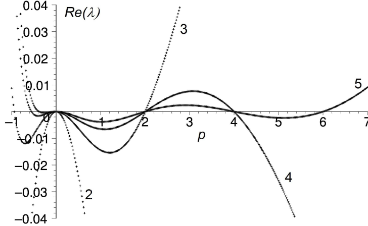
FIGURE 6. The stability with respect to modes m = 2 \dots 5 as a function of p for the rotating ring of Example 2. All modes are stable if and only if p \in (0, 2) .
