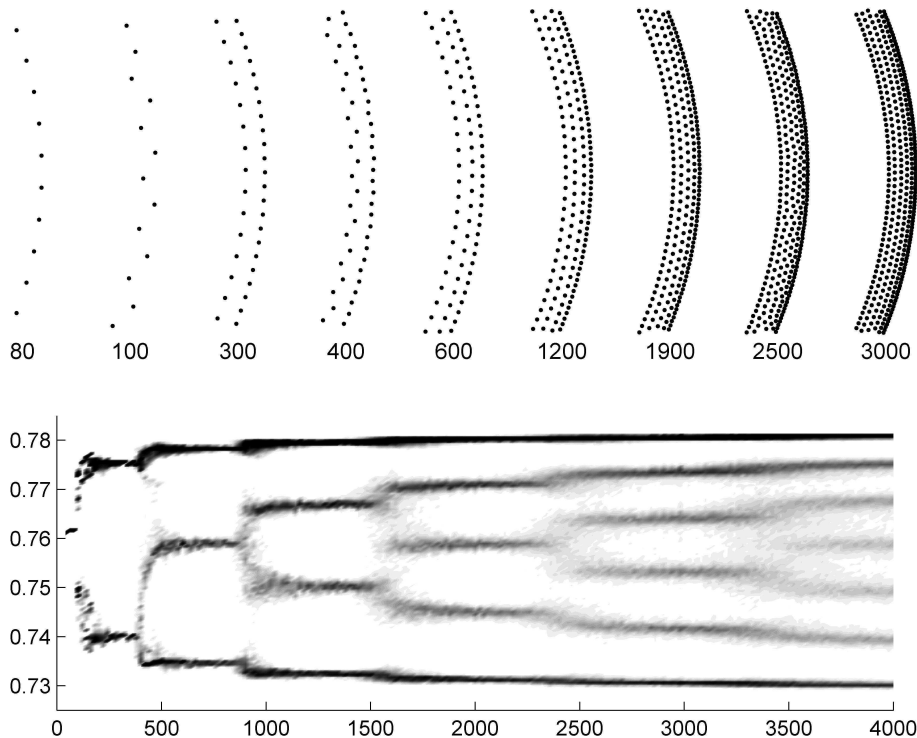
FIGURE 3. Bifurcations of a ring into multiple rings as a function of N , using f(r) = 1 - r^2 + 0.35/r . Top: steady states with N as indicated. These were computed by evolving (2) starting from random initial conditions. A part of the annulus-type solution is shown at t = 25,000 . Bottom: The bifurcation diagram with N on the horizontal axis. The vertical axis shows the distribution of the radii of the particles obtained by computing a steady state up to t = 5000 using random initial conditions.
