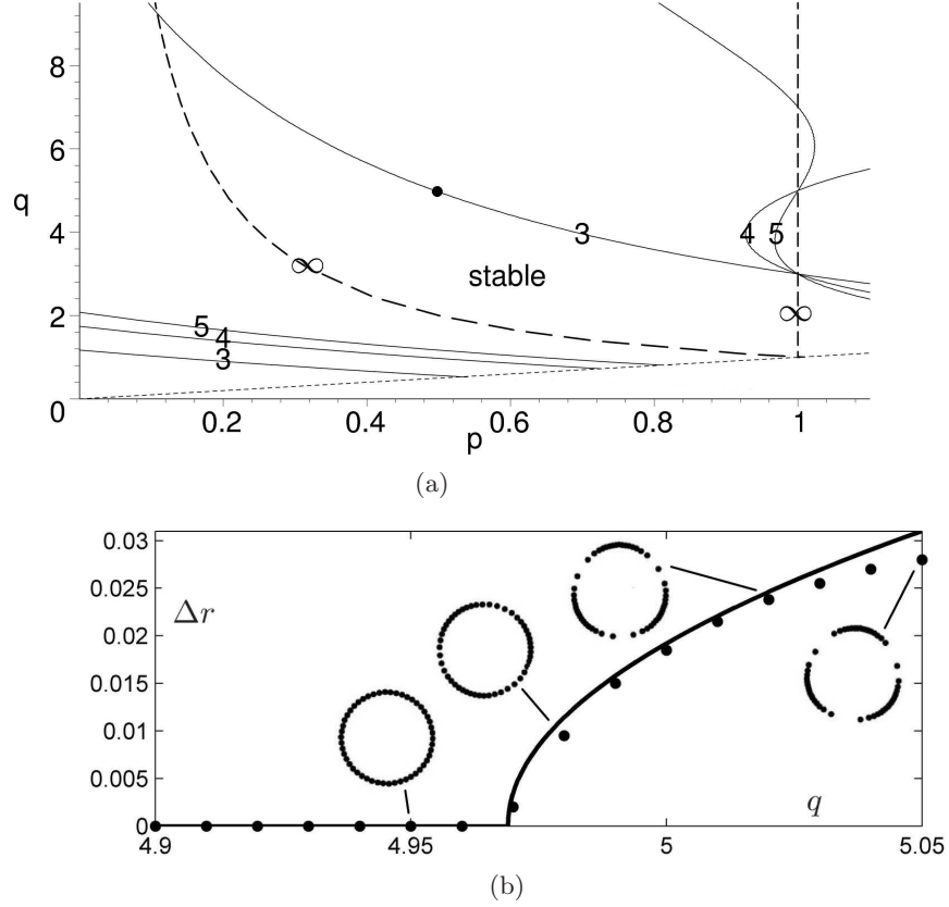
FIGURE 2. (a) Stability region of a ring solution for the force law (24). Instability boundaries corresponding to m = 3, 4, 5 and m = \infty are indicated. Crossing any of these boundaries triggers the corresponding instability. The stable region is bounded by the instability of mode 3 from above and the curve pq = 1 (corresponding to instabilities of modes m \rightarrow \infty ) from below. (b) Bifurcation diagram for interaction force (24) near the dot shown in (a), with p = 0.5 , and as q is varied. The solid curve is derived from weakly nonlinear analysis while the dots are simulations of (2). Reproduced from [17] with authors permission. Copyright (2011) by the American Physical Society.
