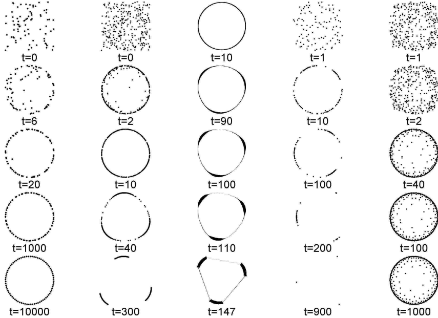
FIGURE 1. Dynamics of (2). First column: f(r) = 1 - r , N = 80 . The equilibrium solution is a stable ring. Second column: f(r) = r^{-0.5} - r^5 , N = 300 . Third column: Simulation of the continuum limit (4) with f as in the second column. Fourth column: f(r) = 1 - r^{2.2} , N = 100 . Fifth column: f(r) = r^{-0.5} - r^{0.5} , N = 300 . Reproduced from [17] with authors permission. Copyright (2011) by the American Physical Society.
