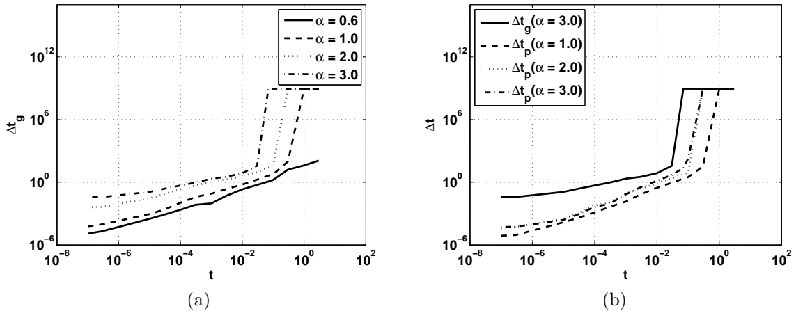
Figure 3: (a) Maximum gradient stable timestep, \Delta t_g . (b) Maximum positivity preserving timesteps, \Delta t_p , computed with various values of \alpha compared with \Delta t_g computed with \alpha = 3.0 .
