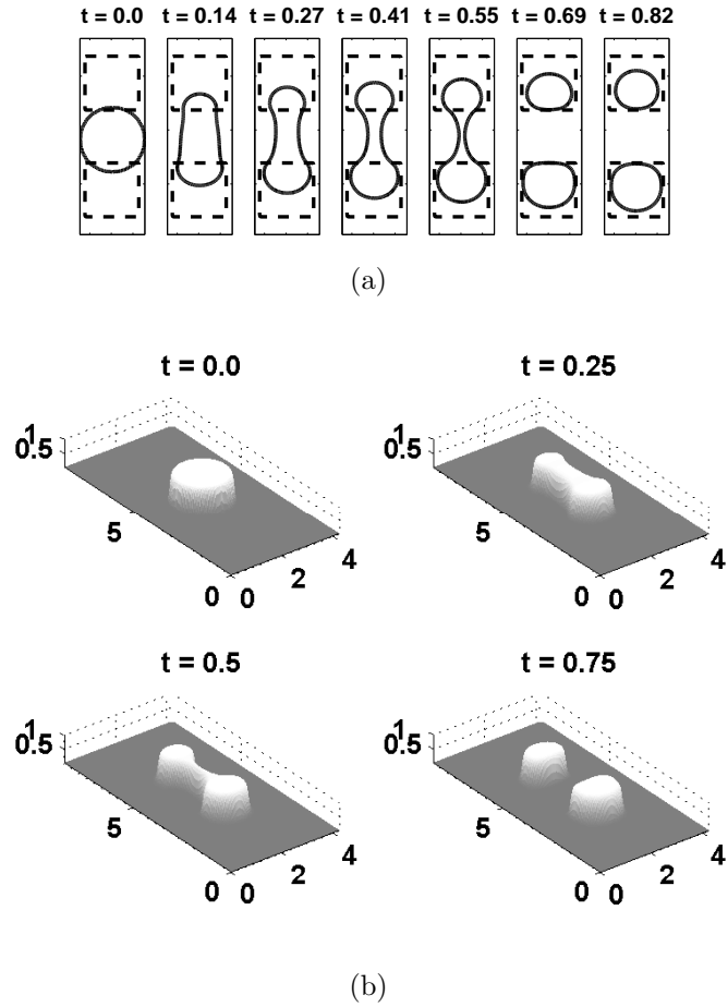
Figure 8: (a) The splitting of a Hele-Shaw drop by two local energies in the dashed squares with \lambda = 3.6 . (b) The 3 dimensional view of the phase field variables.
