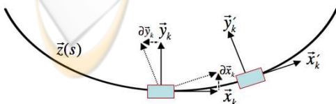
Figure 4: Diagram of the coordinate frame of a micro-car moving along a parametrized path \mathbf{z}(s) .
