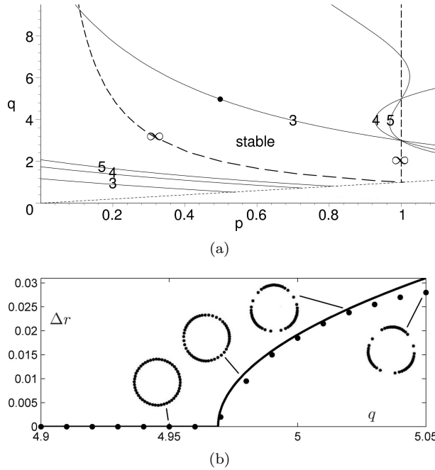
FIG. 4.1. (a) Stability region of a ring solution for the force law (4.1). Instability boundaries corresponding to m=3, 4, 5 and m=\infty are indicated. Crossing any of these boundaries triggers the corresponding instability. The stable region is bounded by the instability of mode 3 from above and the curve pq=1 (corresponding to instabilities of modes m \rightarrow \infty ) from below. (b) Bifurcation diagram for interaction force (4.1) near the dot shown in (a), with p=0.5 , and as q is varied. The solid curve is derived from weakly nonlinear analysis while the dots are simulations of (1.2). Reproduced from [17] with authors permission. Copyright (2011) by the American Physical Society.
