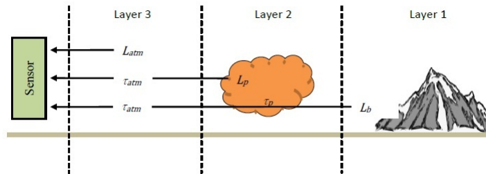
FIGURE 2. Three-layer model depicting the spectral radiance signal received by the long wave infrared sensor.
